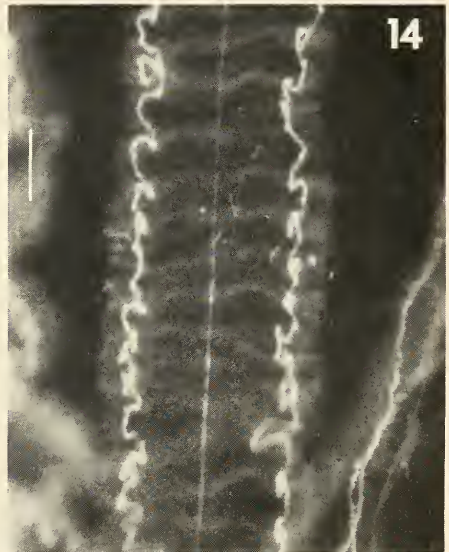
Figs 11-14. Progradungula carraiensis , catching ladder. 11, part of ladder showing non-cribellate support and cribellate catching lines. Scale line 3.0 mm. 12, cribellate line showing dense, fibrillar surface structure. 13-14, structure of cribellate silk line. 13, relaxed; 14, stretched. Scale lines 0.15 mm.
